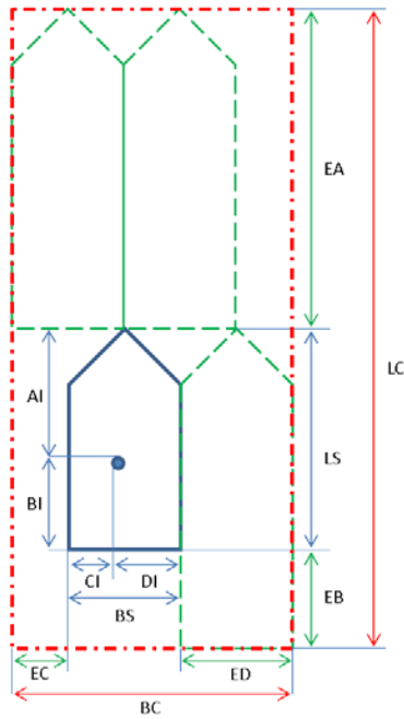
Figure 18: Physical location of GNSS sensor on the ship and in a convoy
