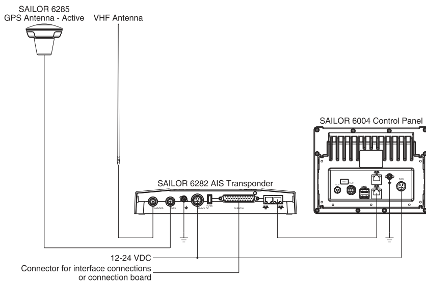
Figure 2: System configuration for the SAILOR 6281 AIS Basic System
