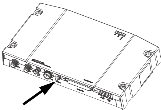
Figure 41: 5 A T fuse in the SAILOR 6282 AIS Transponder
