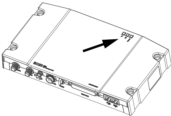
Figure 37: LEDs on the SAILOR 6282 AIS Transponder
